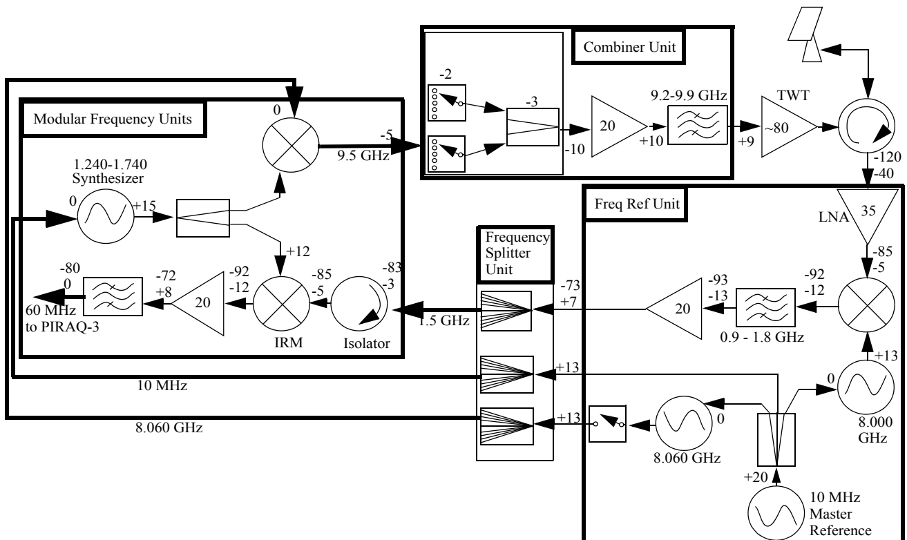
Figure 5. (below) More detailed schematic illustrating frequency generation, combining, and analog processing of received data from one beam.
