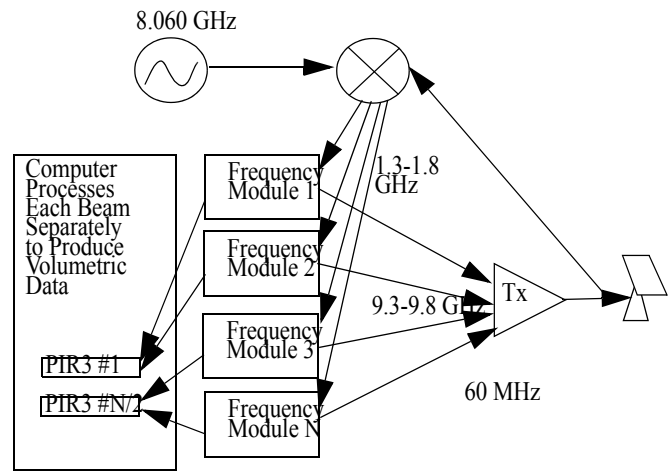
Figure 4. Simplified block diagram illustrating several of the frequency modules and the processing module with PIRAQ-3s.
