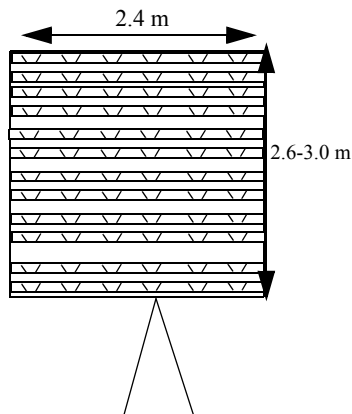
Figure 2. The Rapid-DOW employs a slotted waveguide array to produce several 0.9-1.0° pencil beam. The waveguides will be fed by a sinuous feed oriented vertically.
